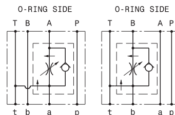
A B Schema idraulico Hydraulic scheme
